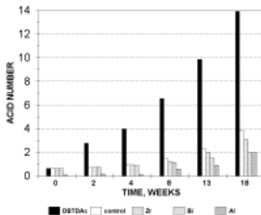
Figure 5 Effect of catalyst on the hydrolytic stability of a polyester in the presence of water at 50°C. Catalysts used
